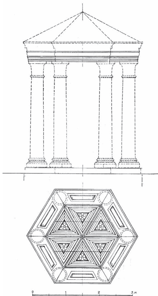
Fig. 20. Hexagonal structure from Serdica (drawing Sava Bobchev 1964).
